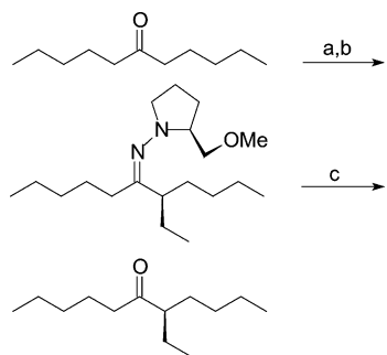
Figure 4. Synthesis of ( R )-5-ethylundecan-6-one ( R -12): (a) SAMP, toluene; (b) LDA, BuI, THF; (c) O 3 .
